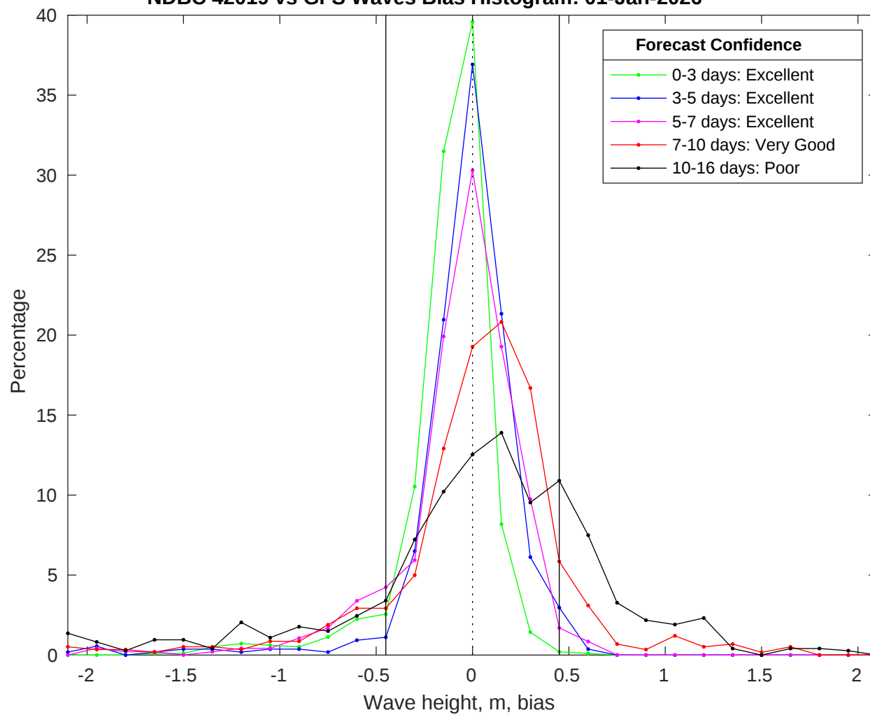
NDBC 42019 vs GFS Waves Bias Histogram: 01-Jan-2026
