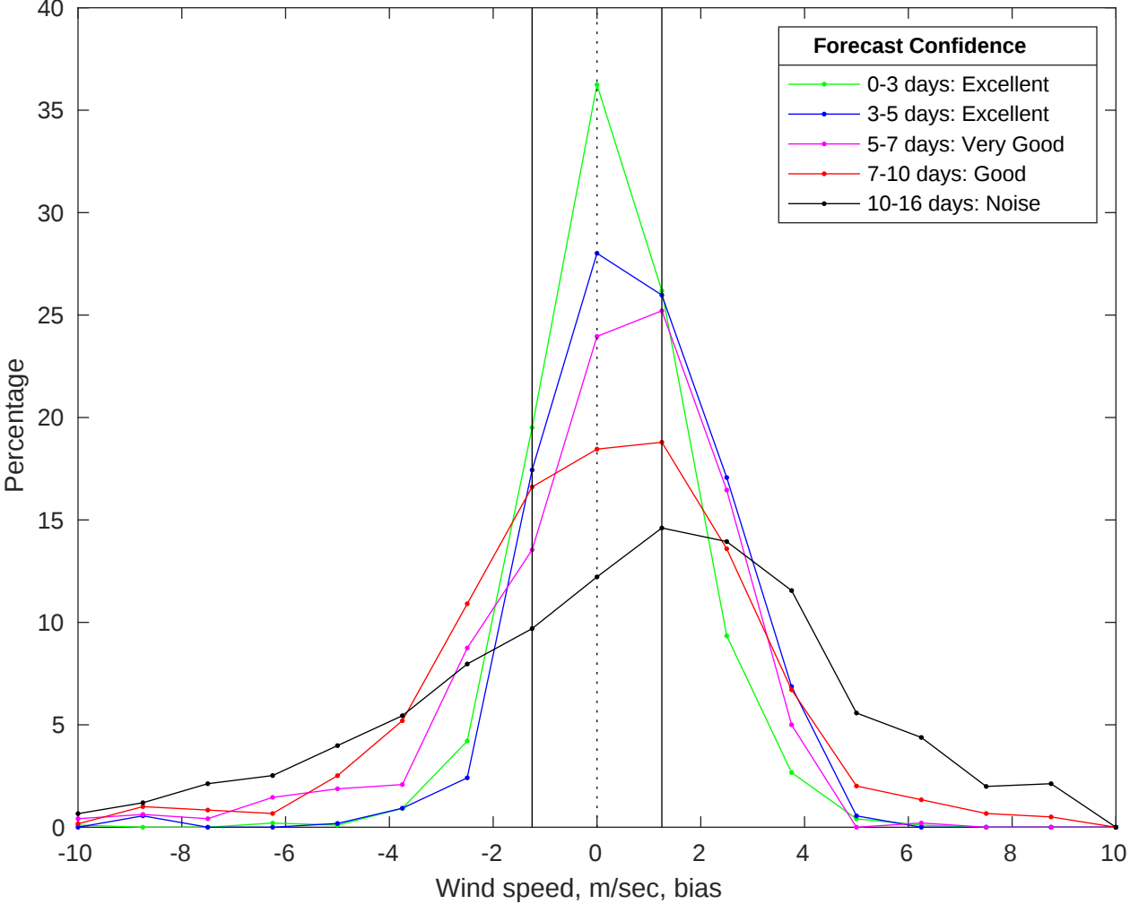
NDBC 42019 vs GFS Winds Bias Histogram: 01-Jan-2026
