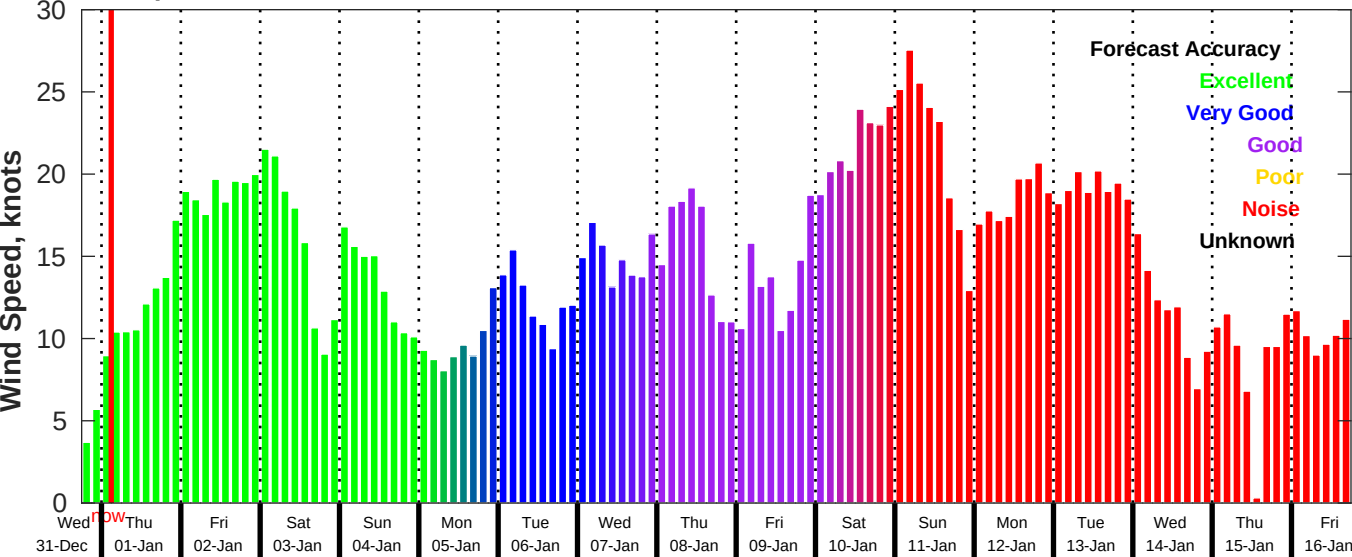
GFS Wind Speed Forecast for NDBC 42019 from 31-Dec-2025 18:00:00 to 16-Jan-2026 18:00:00
