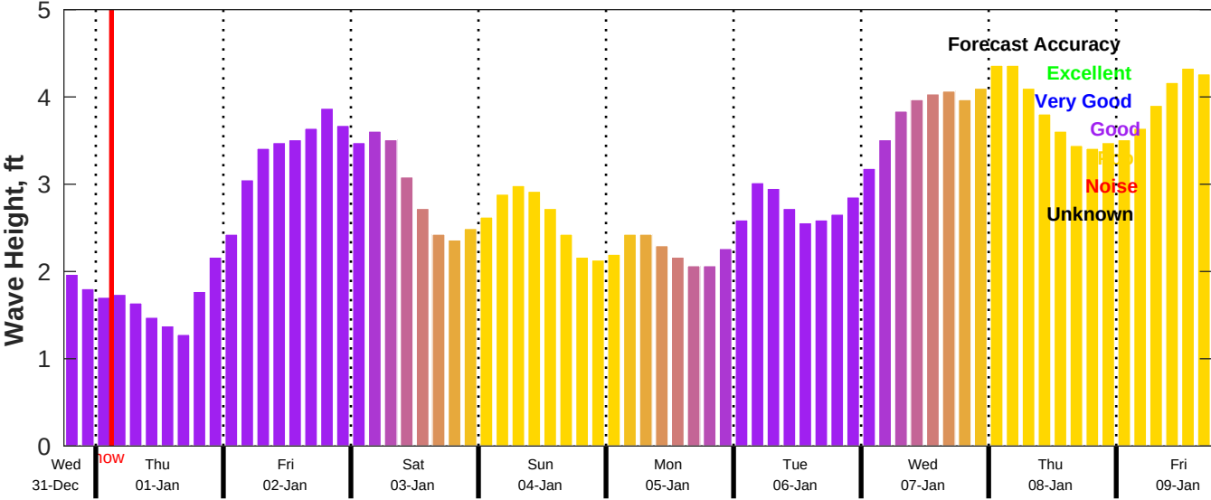
CMEMS Wave Forecast for NDBC 42020 from 31-Dec-2025 18:00:00 to 09-Jan-2026 18:00:00
