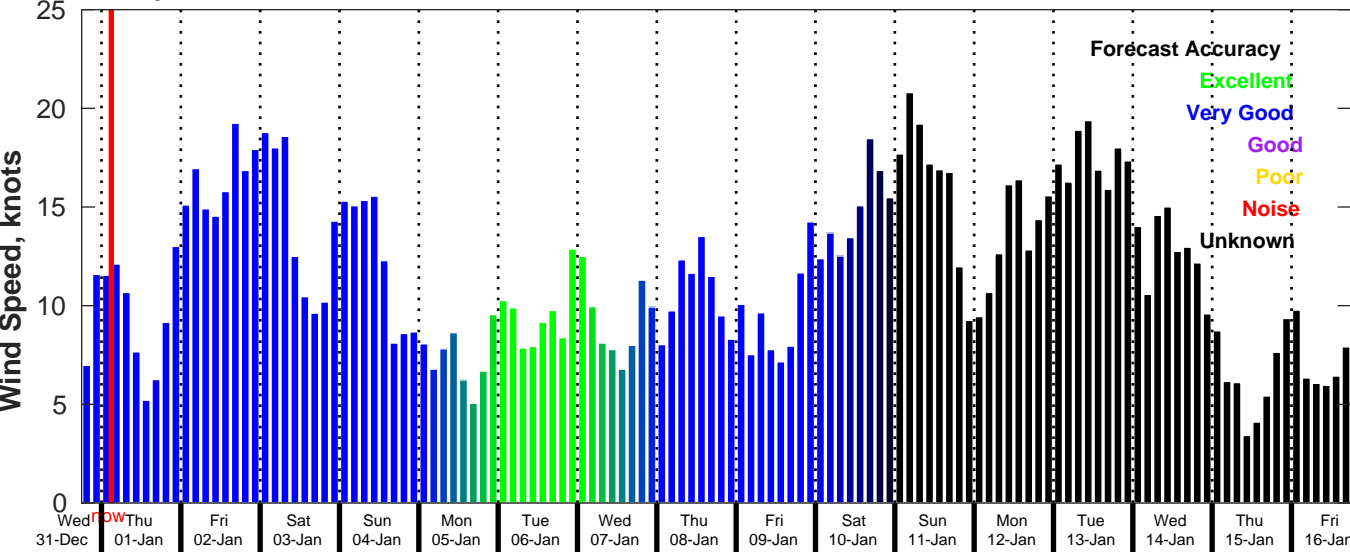
GFS Wind Speed Forecast for NDBC 42035 from 31-Dec-2025 18:00:00 to 16-Jan-2026 18:00:00
