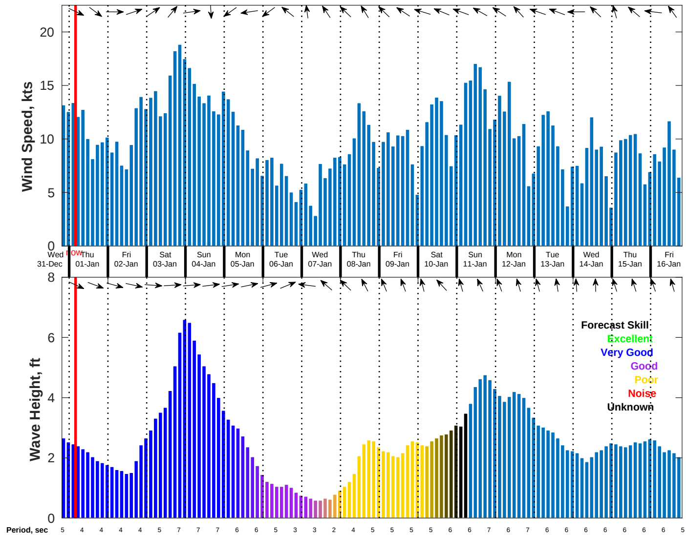
Wind & Wave Forecast for NDBC 42036 from 31-Dec-2025 19:00:00 to 16-Jan-2026 19:00:00
