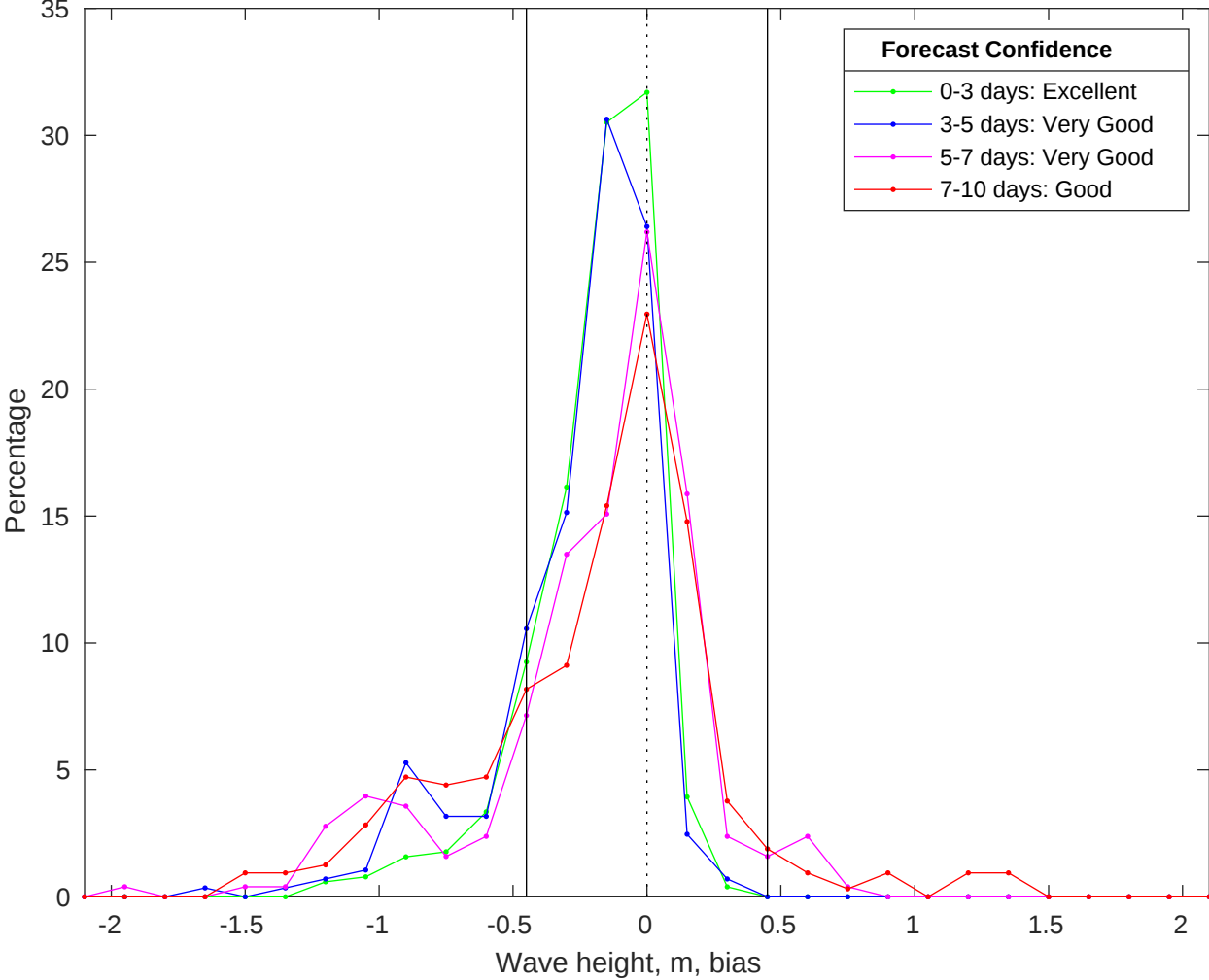
NDBC 42040 vs CMEMS Waves Bias Histogram: 01-Jan-2026
