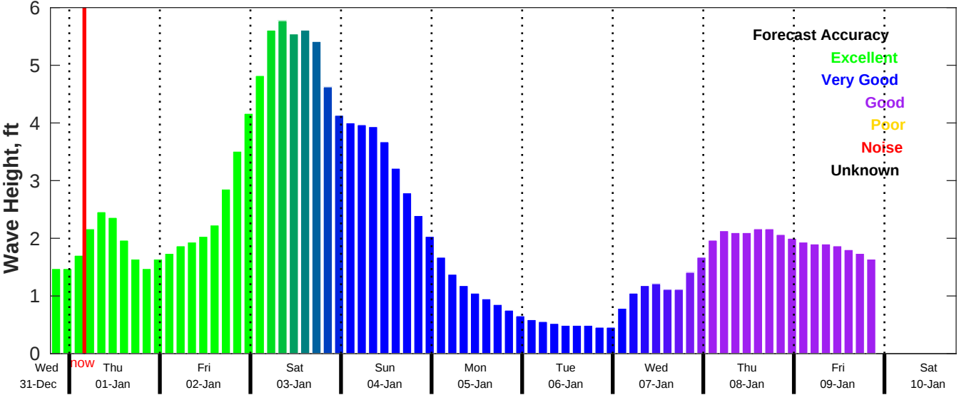
CMEMS Wave Forecast for NDBC 42040 from 31-Dec-2025 19:00:00 to 10-Jan-2026 19:00:00
