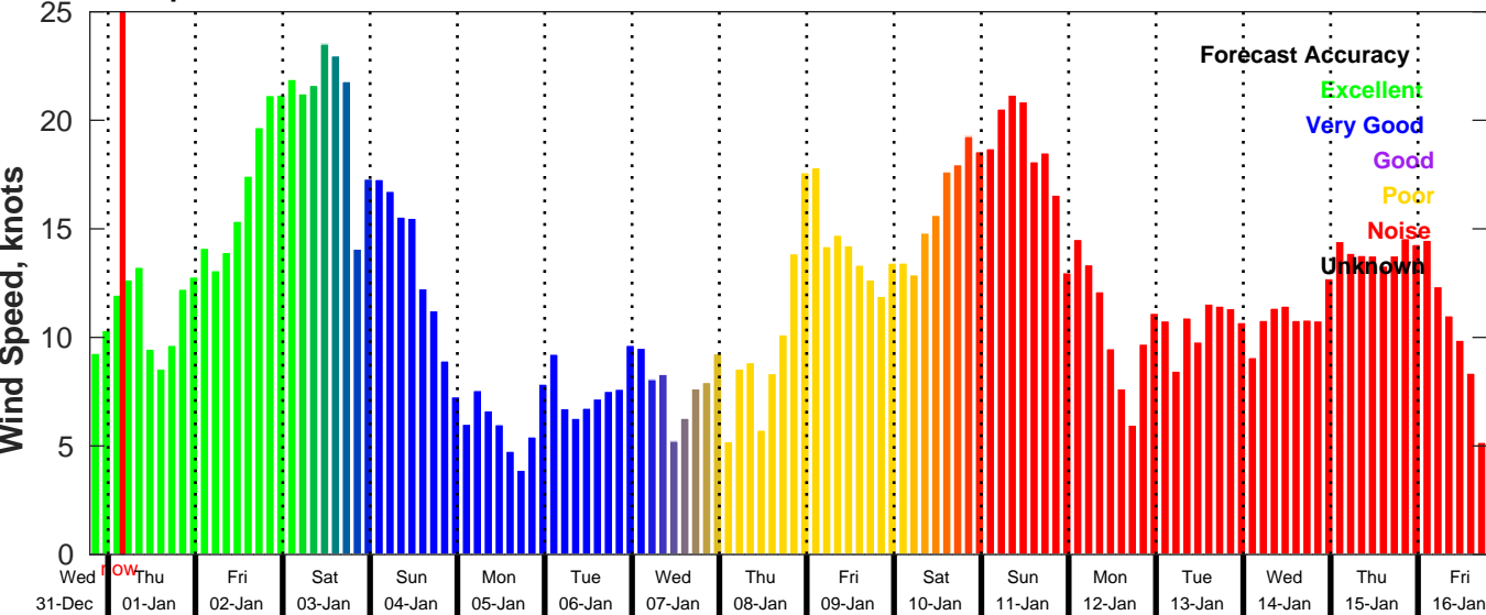
GFS Wind Speed Forecast for NDBC 42040 from 31-Dec-2025 19:00:00 to 16-Jan-2026 19:00:00
