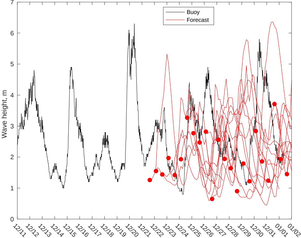
NDBC 44008 vs GFS Waves: 10 to 16 day forecast
