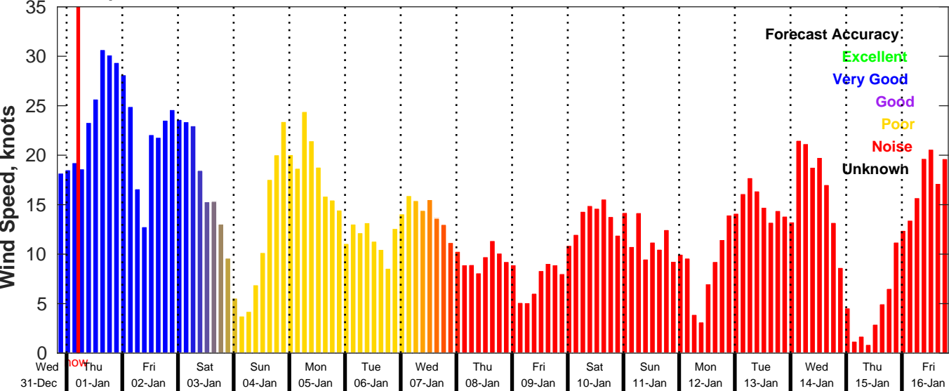
GFS Wind Speed Forecast for NDBC 44008 from 31-Dec-2025 20:00:00 to 16-Jan-2026 20:00:00
