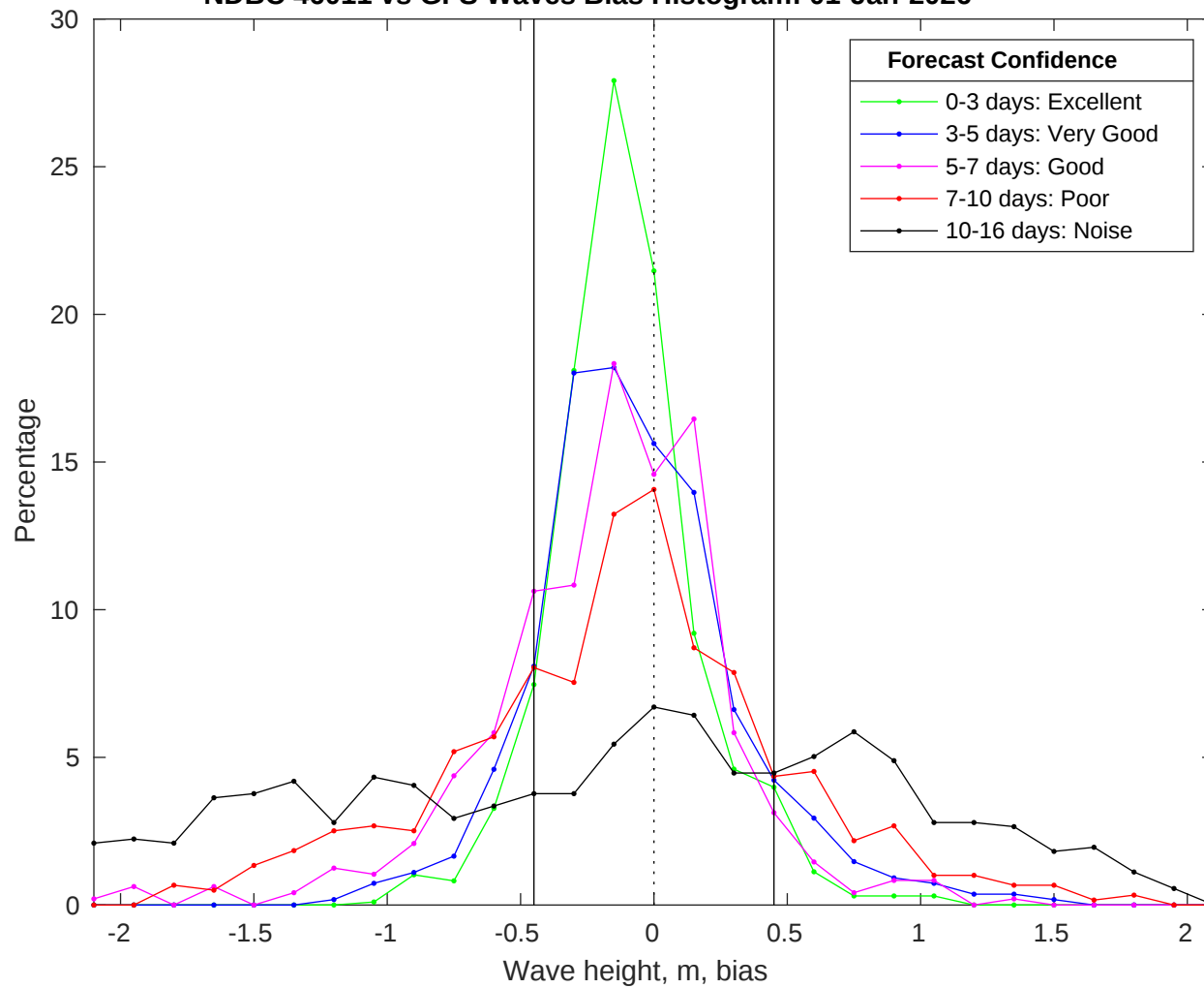
NDBC 46011 vs GFS Waves Bias Histogram: 01-Jan-2026
