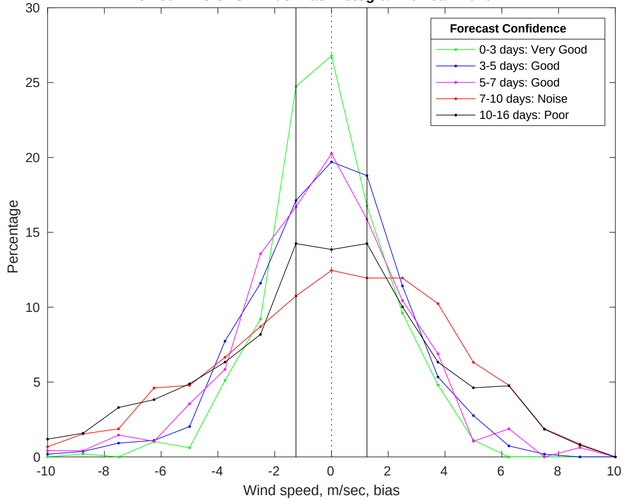
NDBC 46011 vs GFS Winds Bias Histogram: 01-Jan-2026
