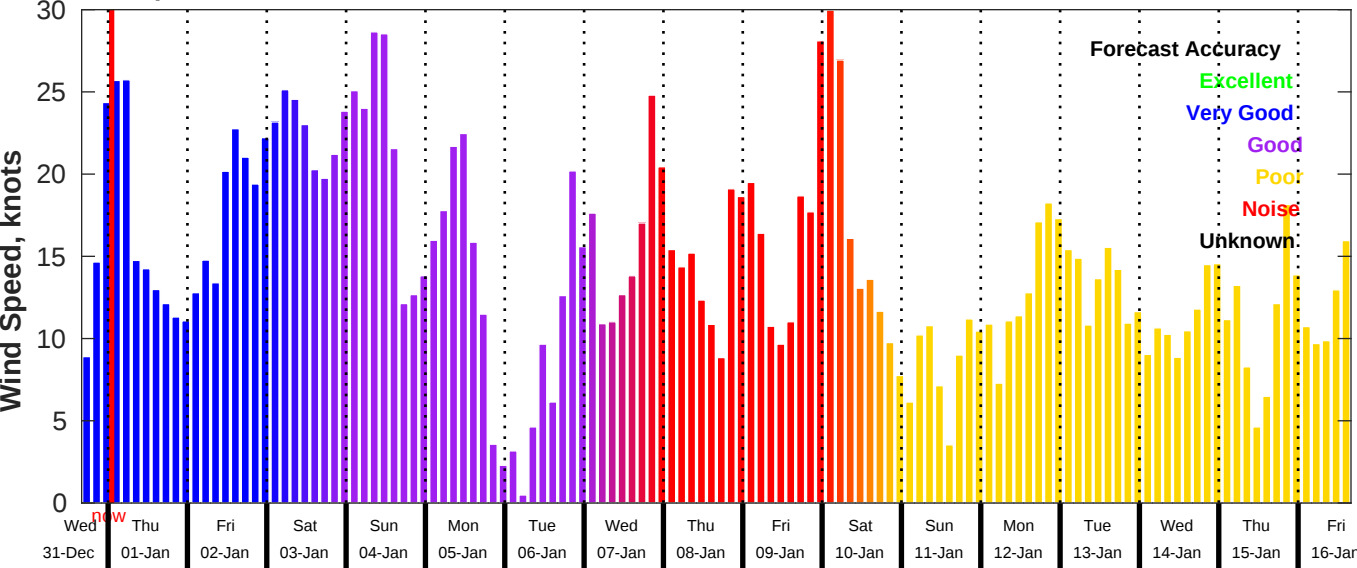
GFS Wind Speed Forecast for NDBC 46011 from 31-Dec-2025 16:00:00 to 16-Jan-2026 16:00:00
