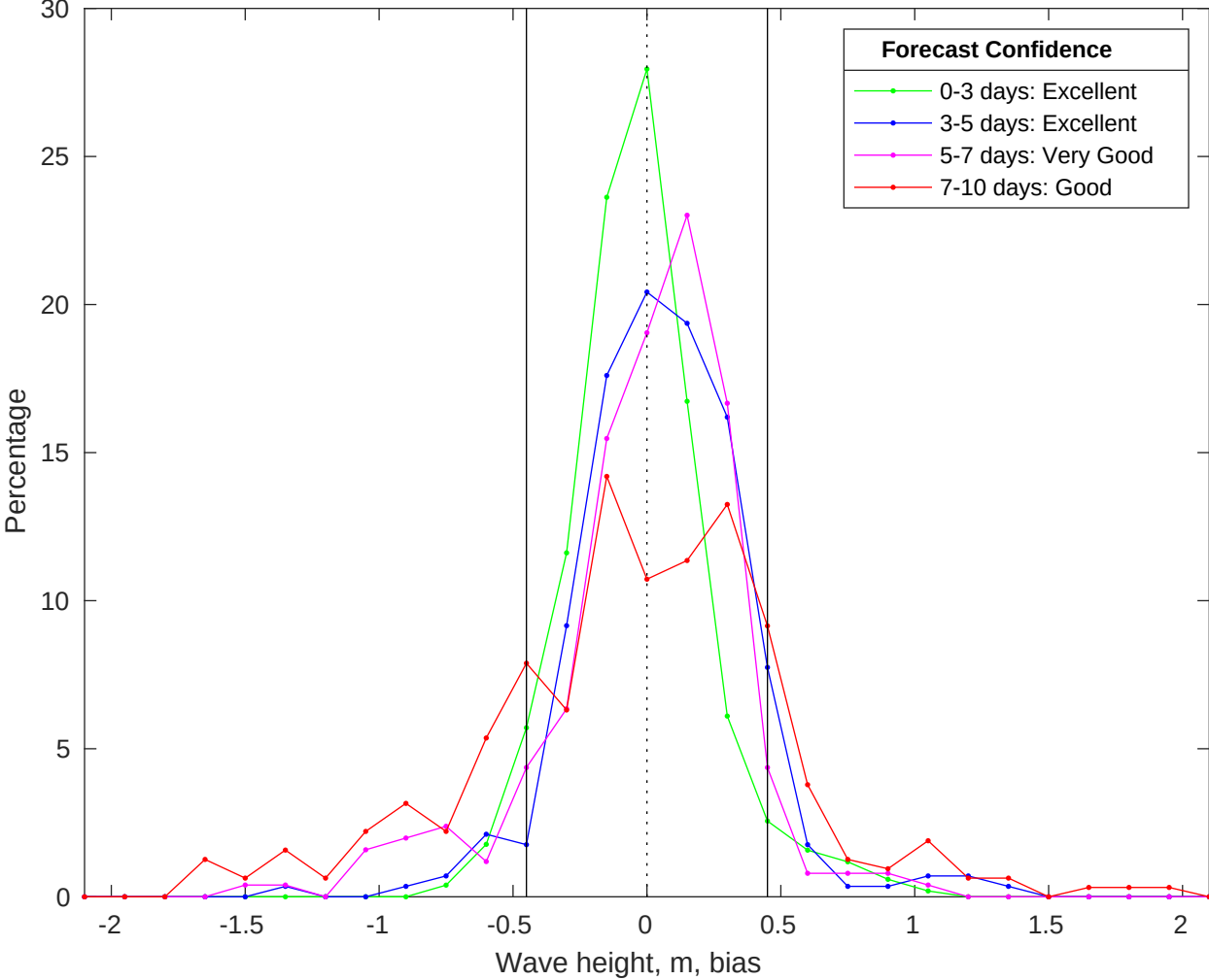
NDBC 46028 vs CMEMS Waves Bias Histogram: 01-Jan-2026
