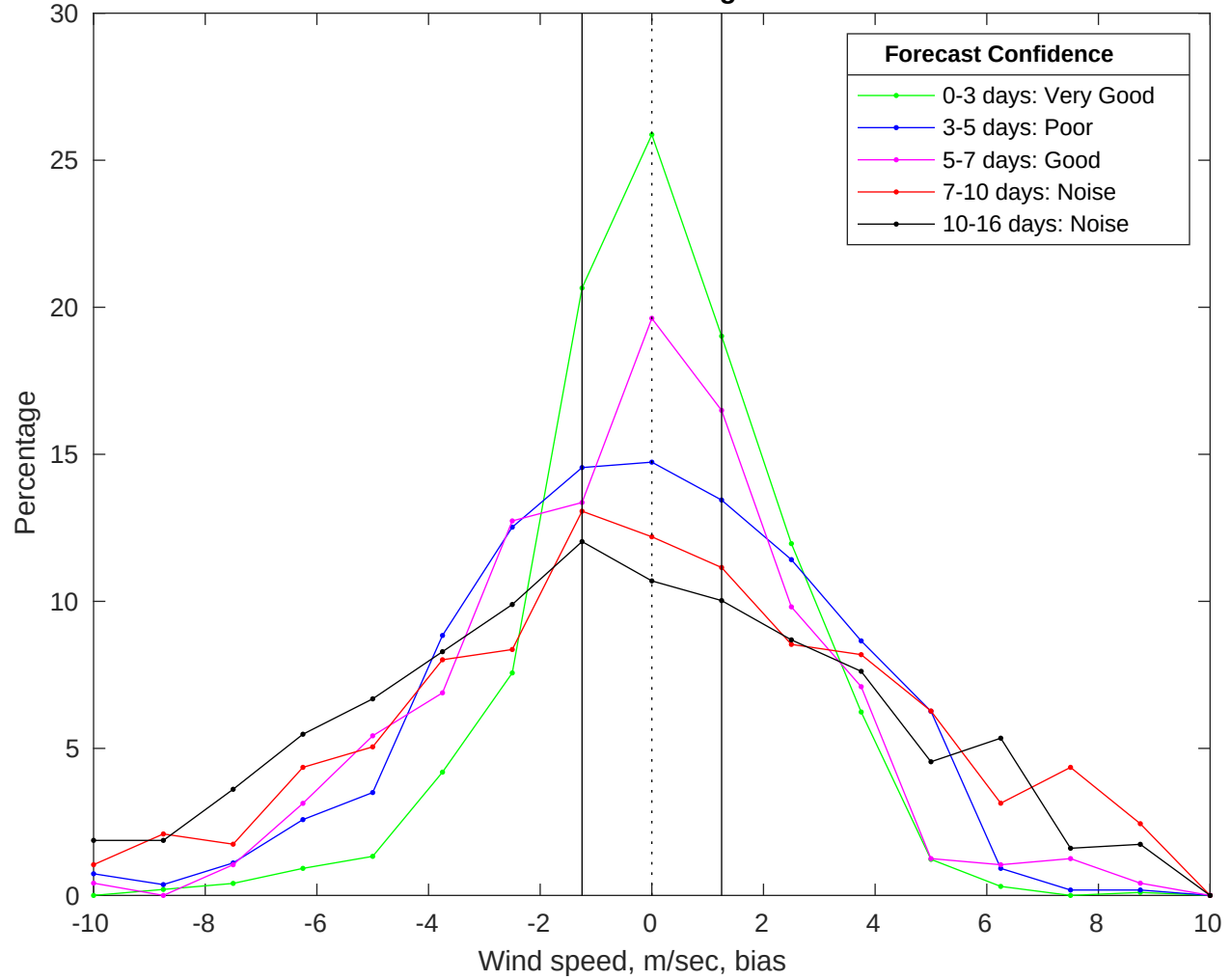
NDBC 46028 vs GFS Winds Bias Histogram: 01-Jan-2026
