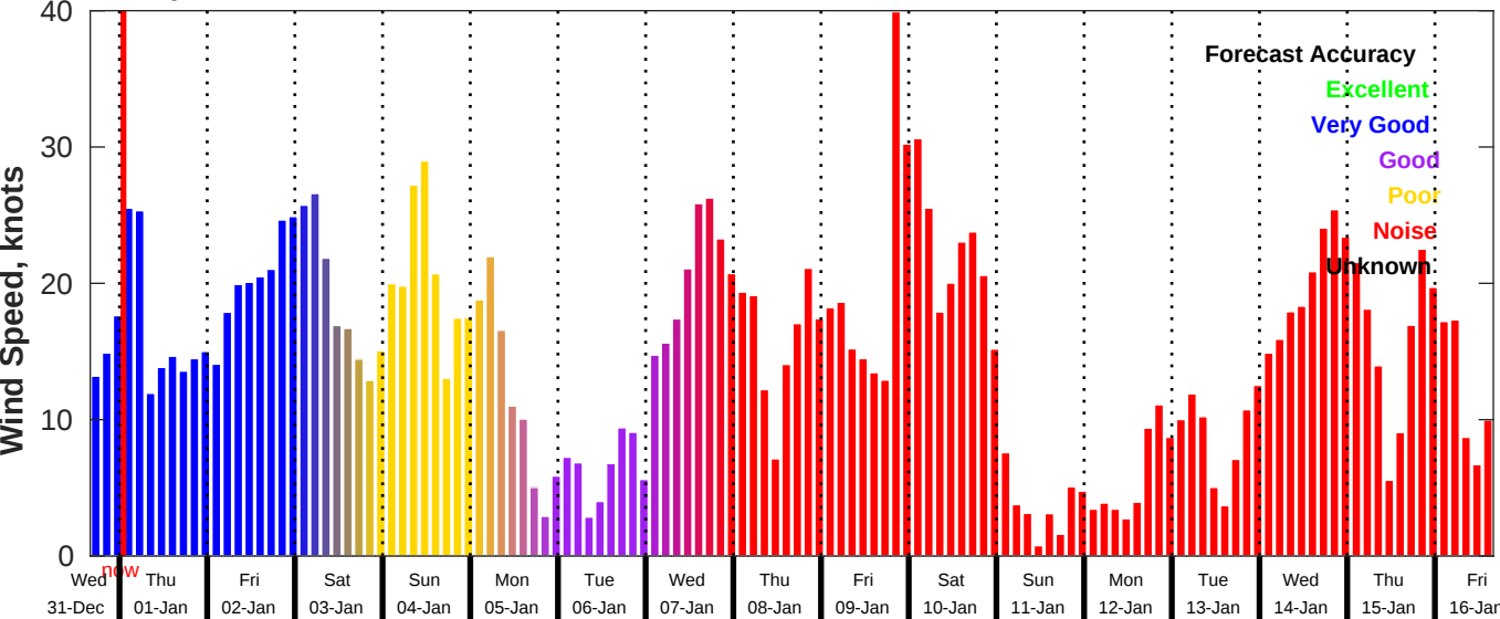
GFS Wind Speed Forecast for NDBC 46028 from 31-Dec-2025 16:00:00 to 16-Jan-2026 16:00:00
