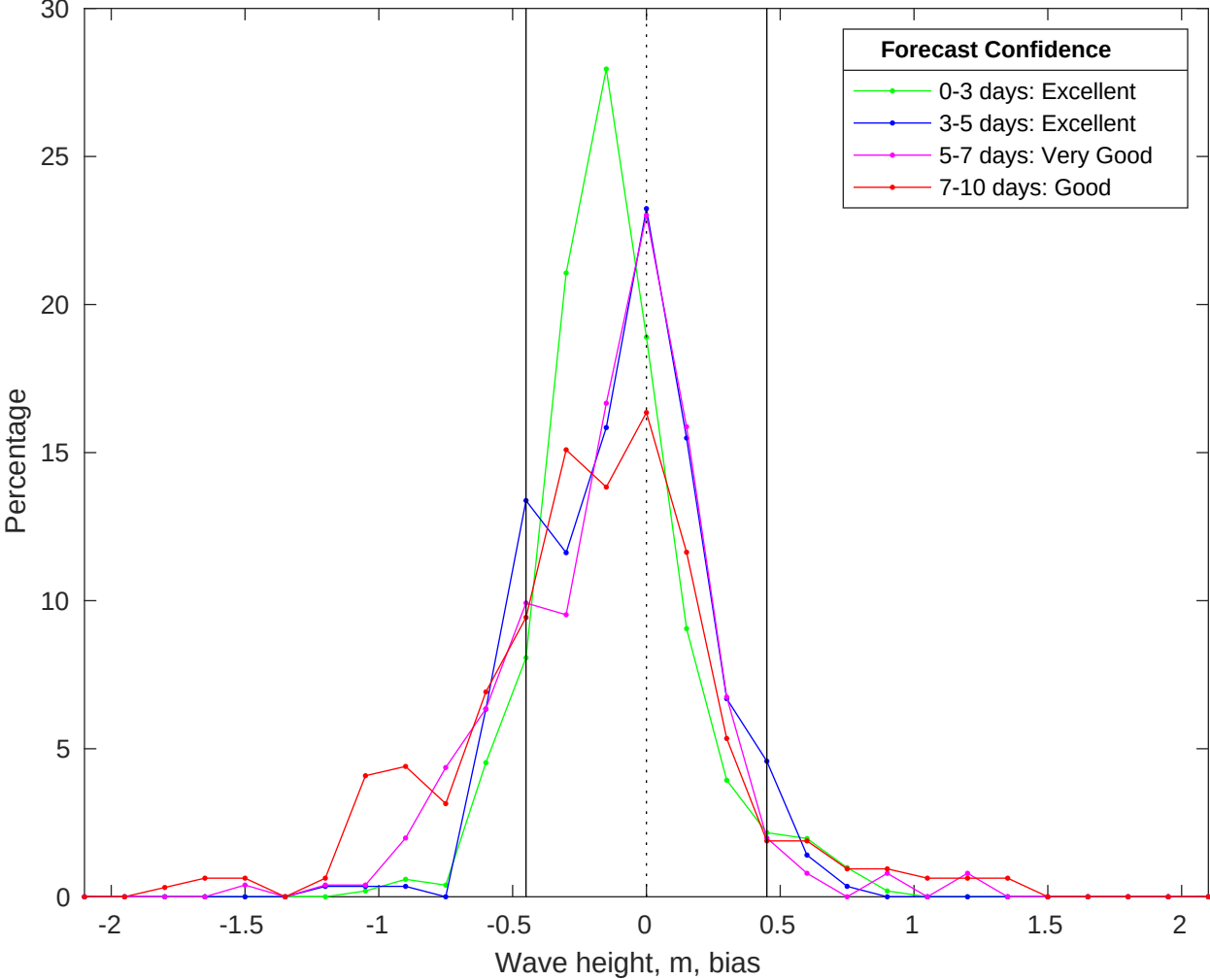
NDBC 46054 vs CMEMS Waves Bias Histogram: 01-Jan-2026
