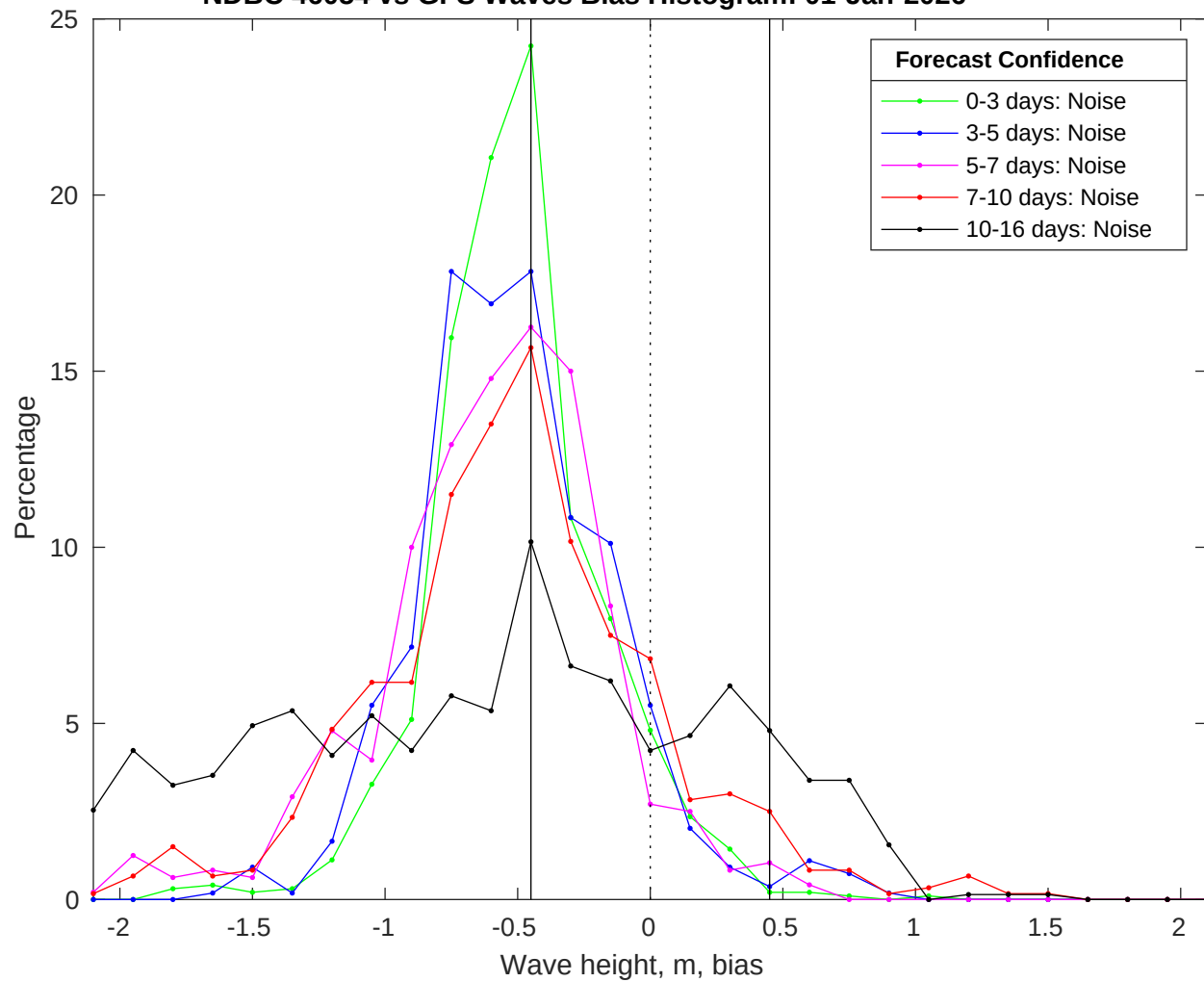
NDBC 46054 vs GFS Waves Bias Histogram: 01-Jan-2026
