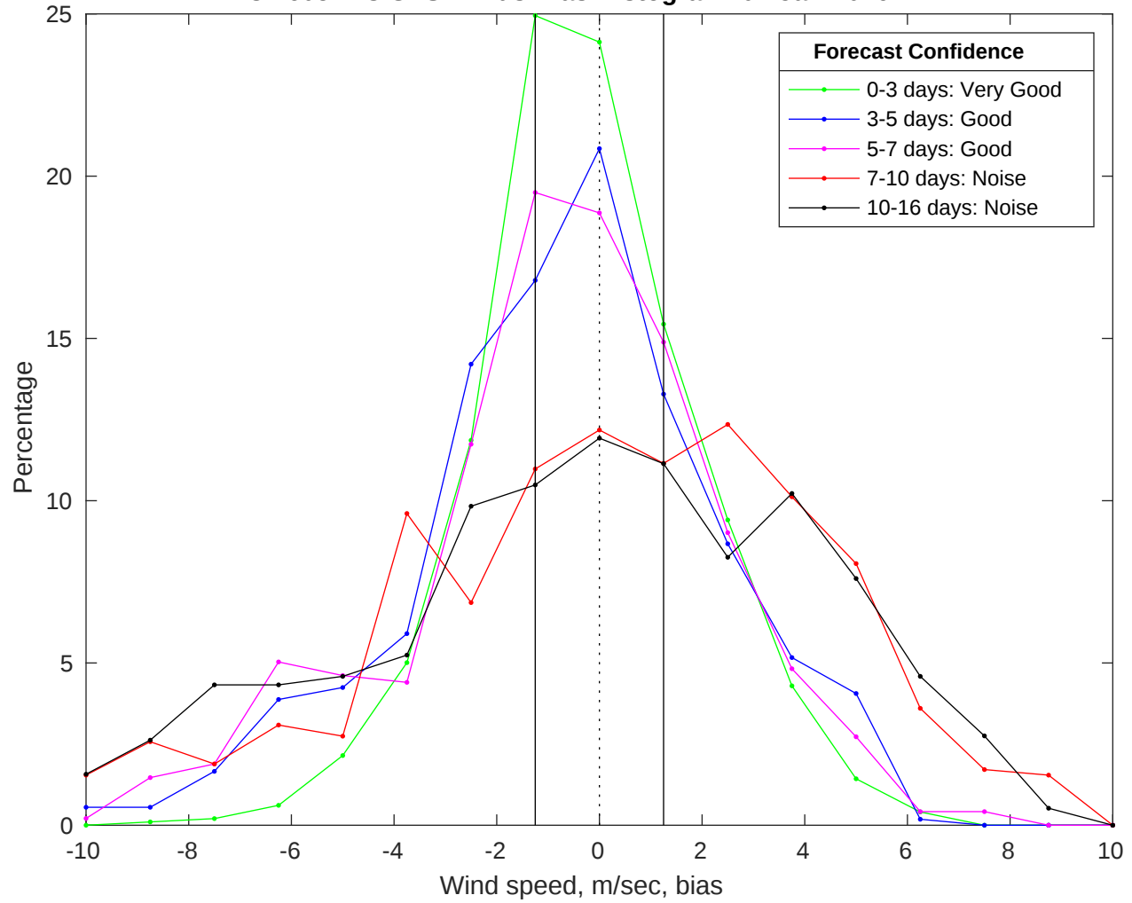
NDBC 46054 vs GFS Winds Bias Histogram: 01-Jan-2026
