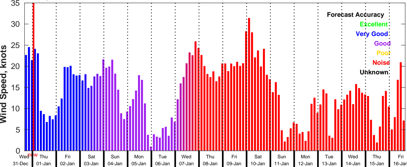
GFS Wind Speed Forecast for NDBC 46054 from 31-Dec-2025 16:00:00 to 16-Jan-2026 16:00:00
