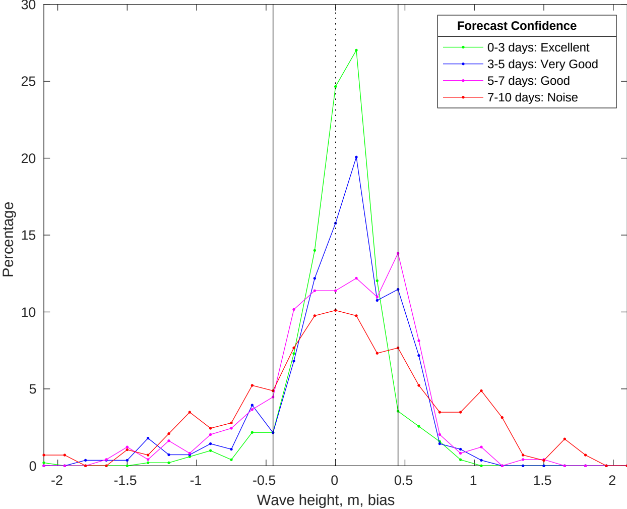
NDBC 46059 vs CMEMS Waves Bias Histogram: 01-Jan-2026
