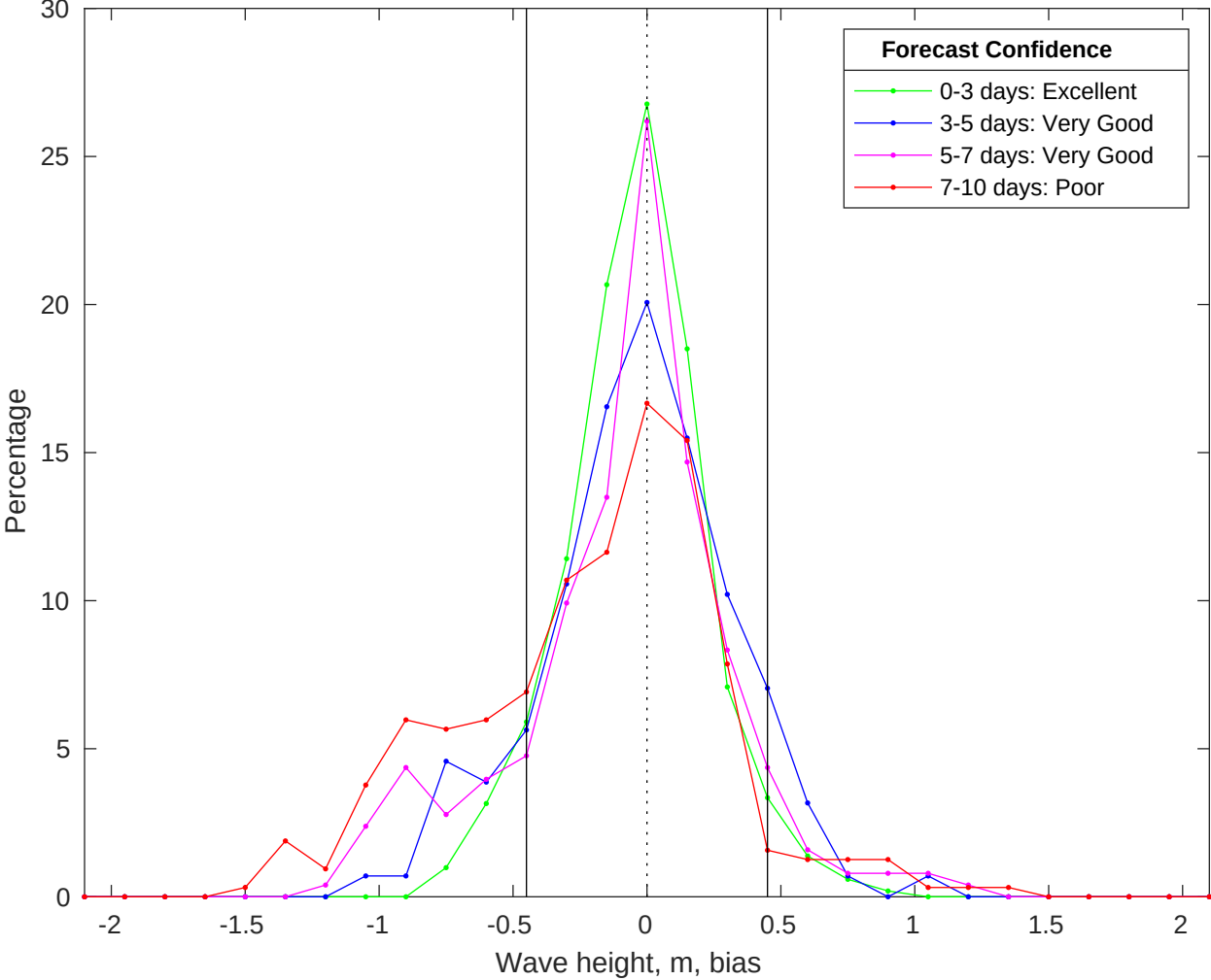
NDBC 46069 vs CMEMS Waves Bias Histogram: 01-Jan-2026
