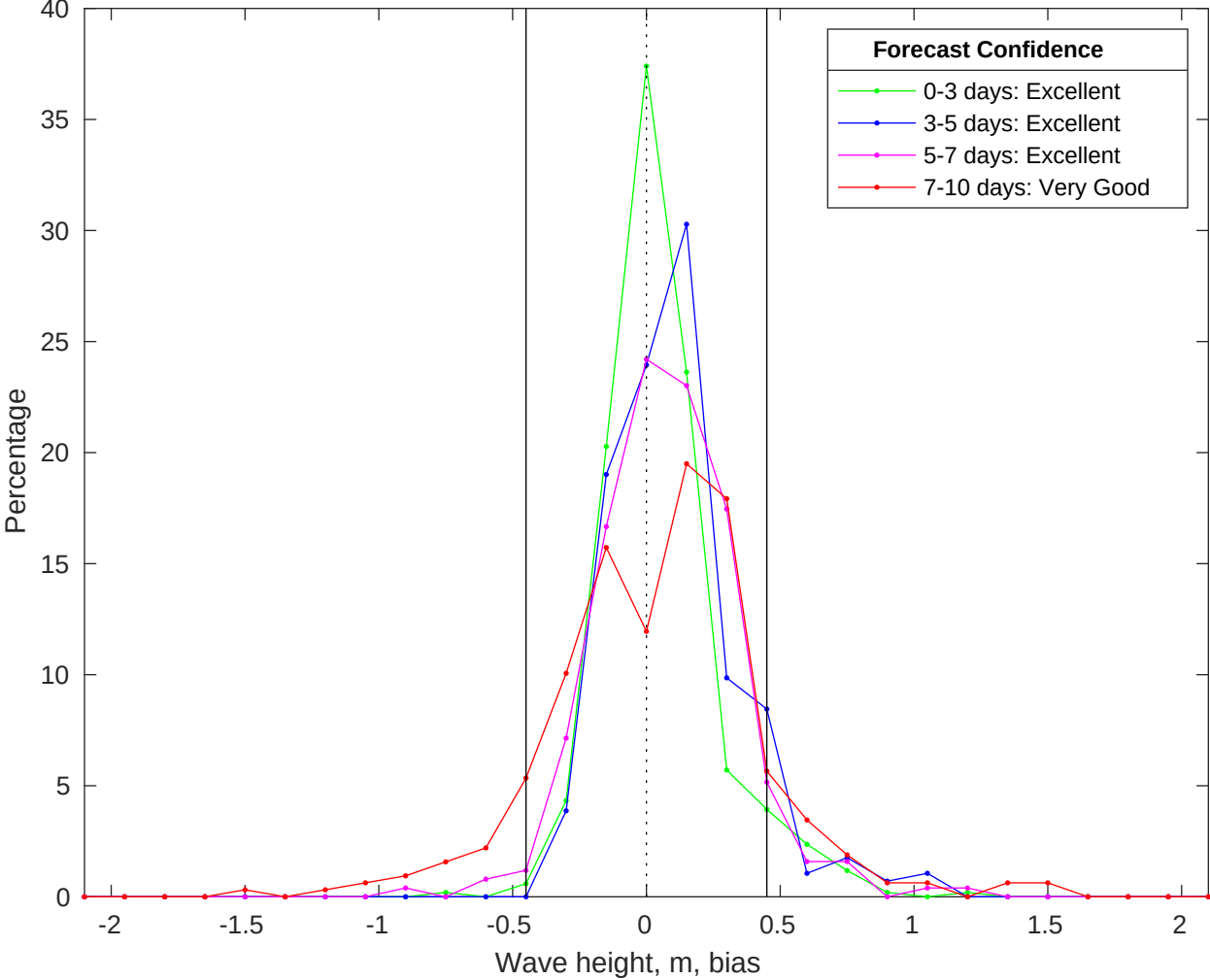
NDBC 46215 vs CMEMS Waves Bias Histogram: 01-Jan-2026
