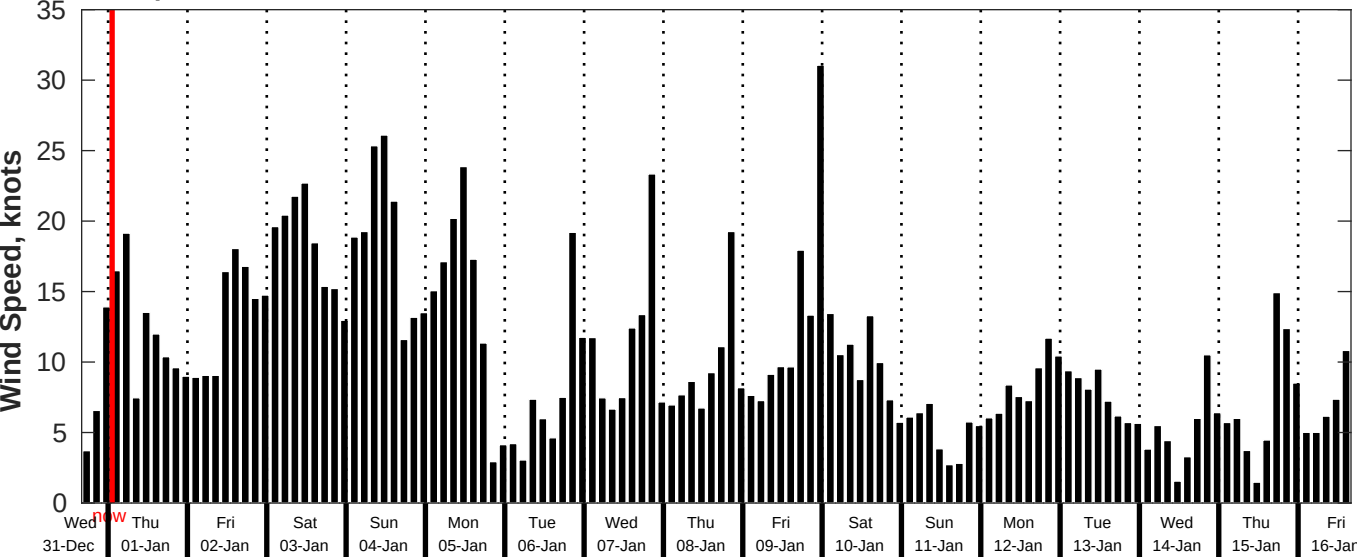
GFS Wind Speed Forecast for NDBC 46215 from 31-Dec-2025 16:00:00 to 16-Jan-2026 16:00:00
