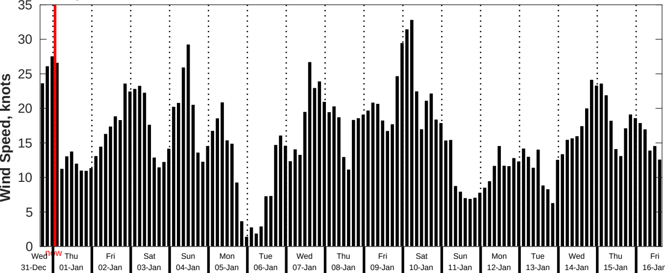
GFS Wind Speed Forecast for NDBC 46259 from 31-Dec-2025 16:00:00 to 16-Jan-2026 16:00:00
