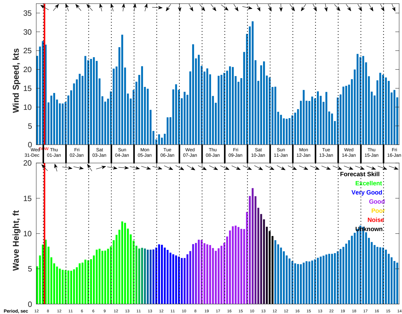
Wind & Wave Forecast for NDBC 46259 from 31-Dec-2025 16:00:00 to 16-Jan-2026 16:00:00
