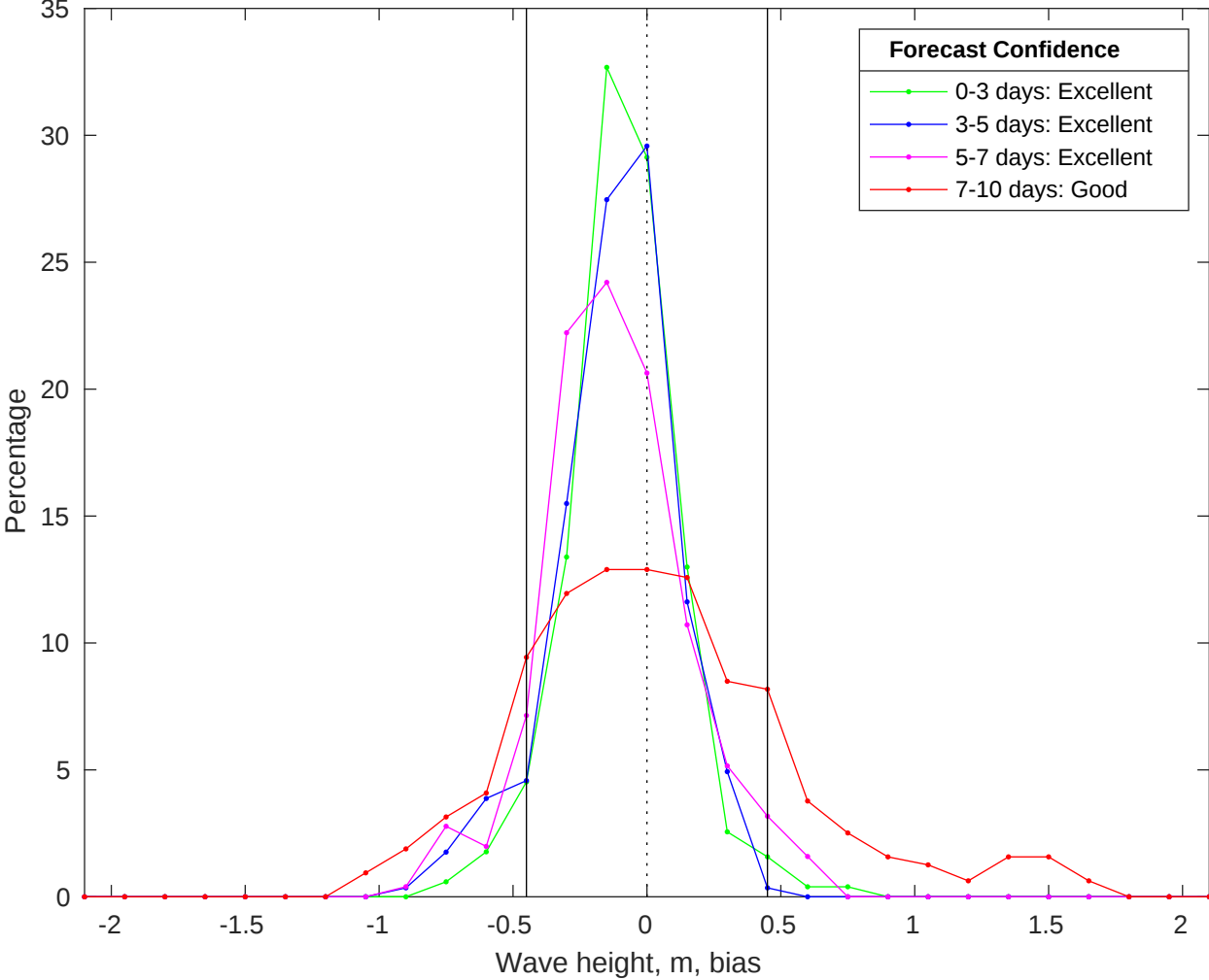
NDBC 51000 vs CMEMS Waves Bias Histogram: 01-Jan-2026
