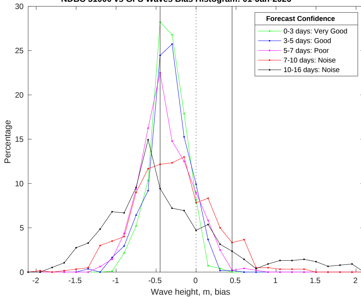
NDBC 51000 vs GFS Waves Bias Histogram: 01-Jan-2026
