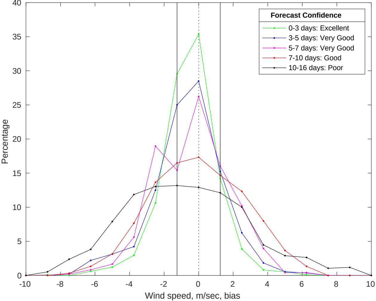
NDBC 51000 vs GFS Winds Bias Histogram: 01-Jan-2026
