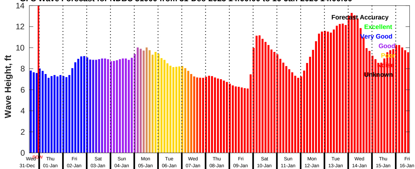
GFS Wave Forecast for NDBC 51000 from 31-Dec-2025 14:00:00 to 16-Jan-2026 14:00:00
