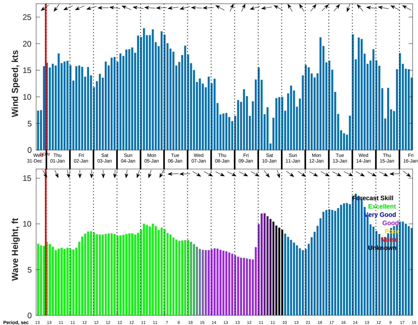
Wind & Wave Forecast for NDBC 51000 from 31-Dec-2025 14:00:00 to 16-Jan-2026 14:00:00
