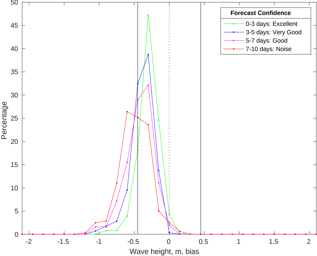
NDBC 51209 vs CMEMS Waves Bias Histogram: 01-Jan-2026
