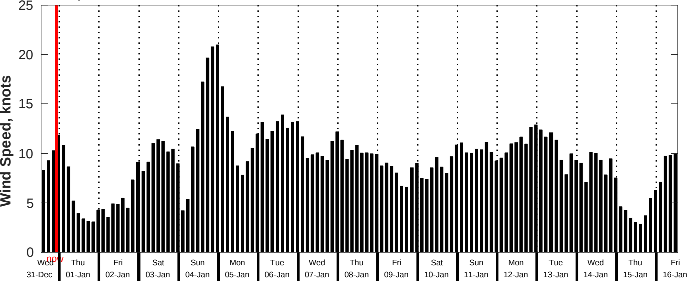
GFS Wind Speed Forecast for NDBC 51209 from 31-Dec-2025 13:00:00 to 16-Jan-2026 13:00:00
