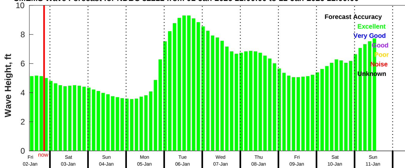
CMEMS Wave Forecast for NDBC 52211 from 01-Jan-2026 11:00:00 to 11-Jan-2026 11:00:00
