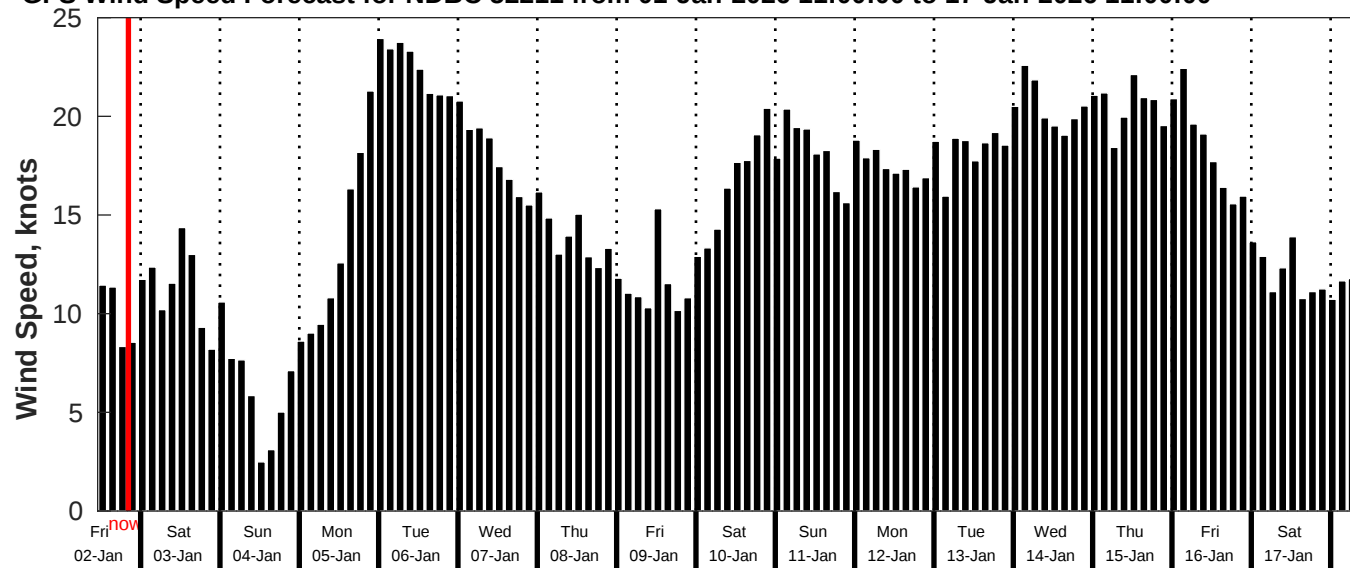
GFS Wind Speed Forecast for NDBC 52211 from 01-Jan-2026 11:00:00 to 17-Jan-2026 11:00:00
