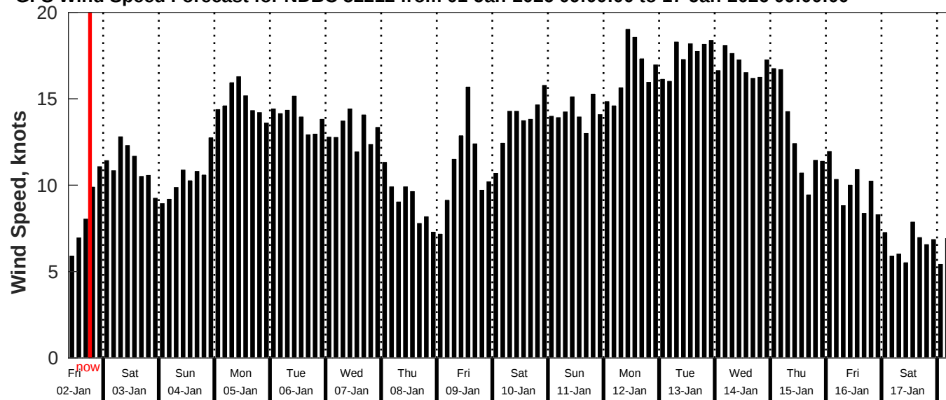
GFS Wind Speed Forecast for NDBC 52212 from 01-Jan-2026 09:00:00 to 17-Jan-2026 09:00:00
