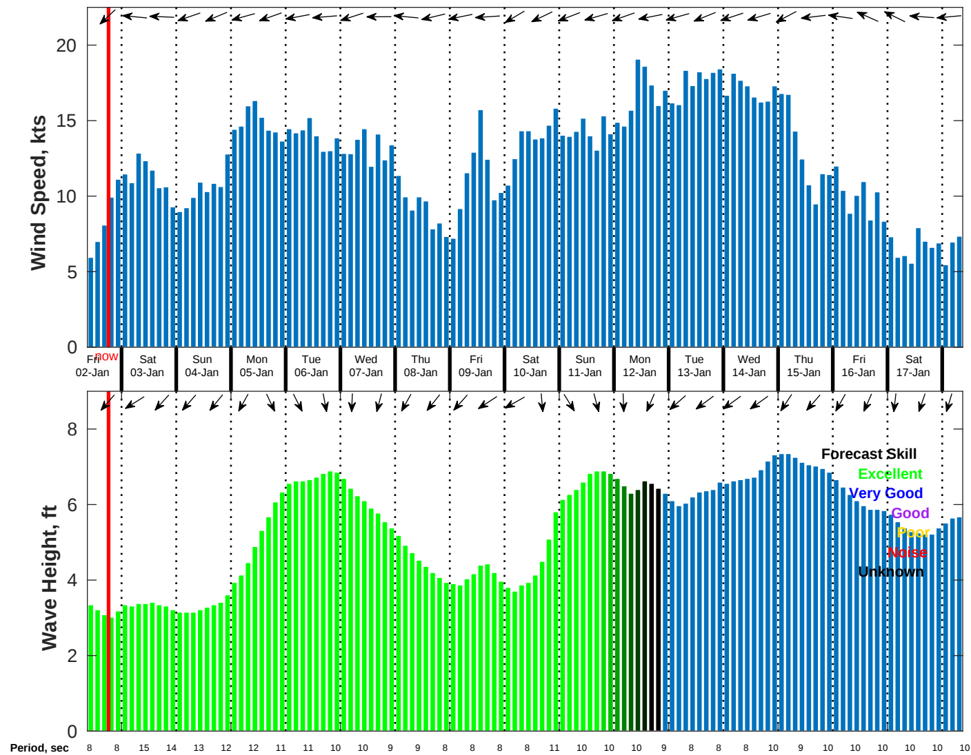
Wind & Wave Forecast for NDBC 52212 from 01-Jan-2026 09:00:00 to 17-Jan-2026 09:00:00
