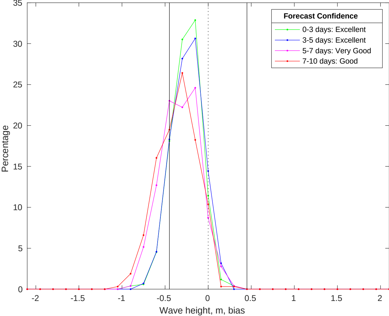
NDBC 52213 vs CMEMS Waves Bias Histogram: 01-Jan-2026
