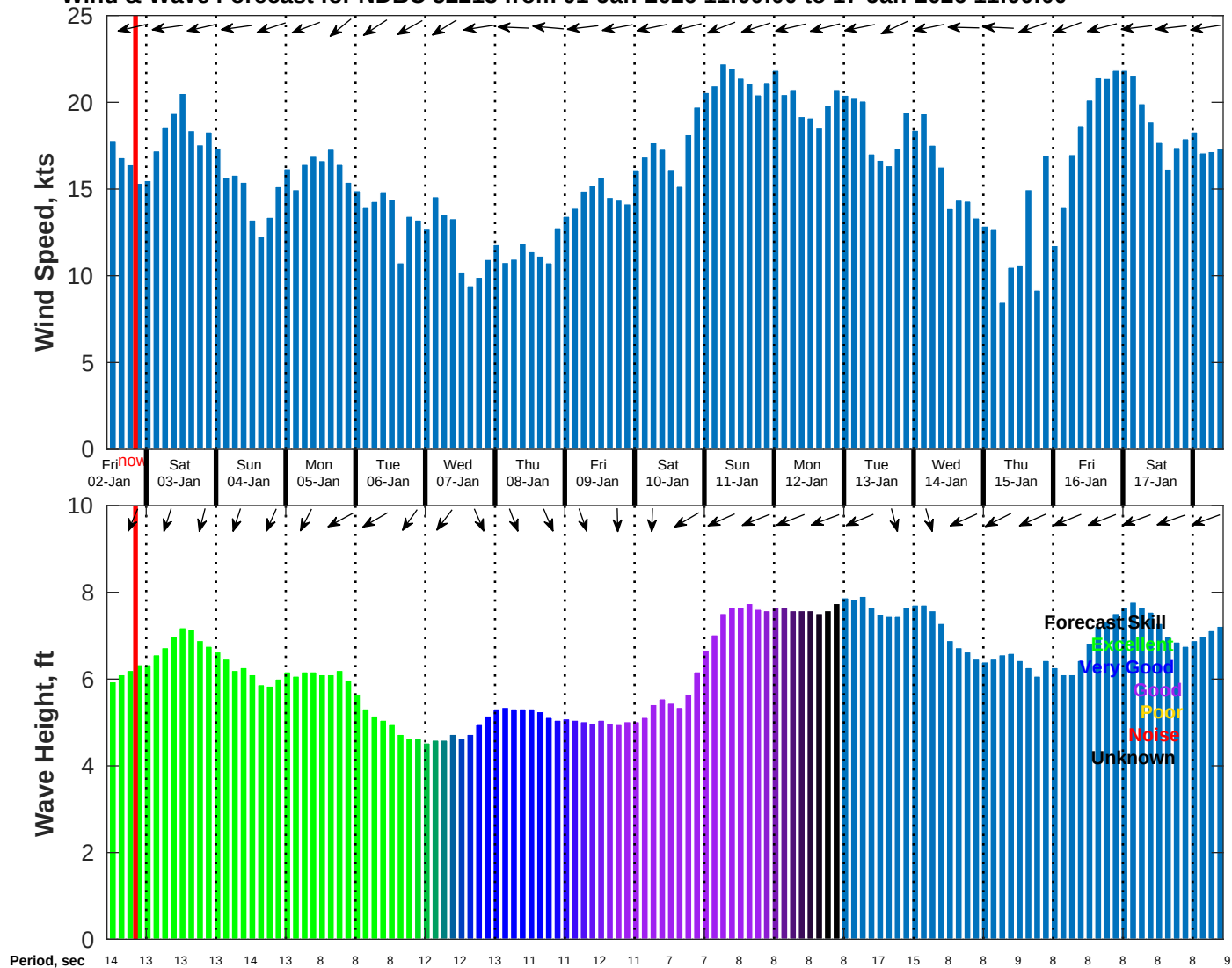
Wind & Wave Forecast for NDBC 52213 from 01-Jan-2026 11:00:00 to 17-Jan-2026 11:00:00
