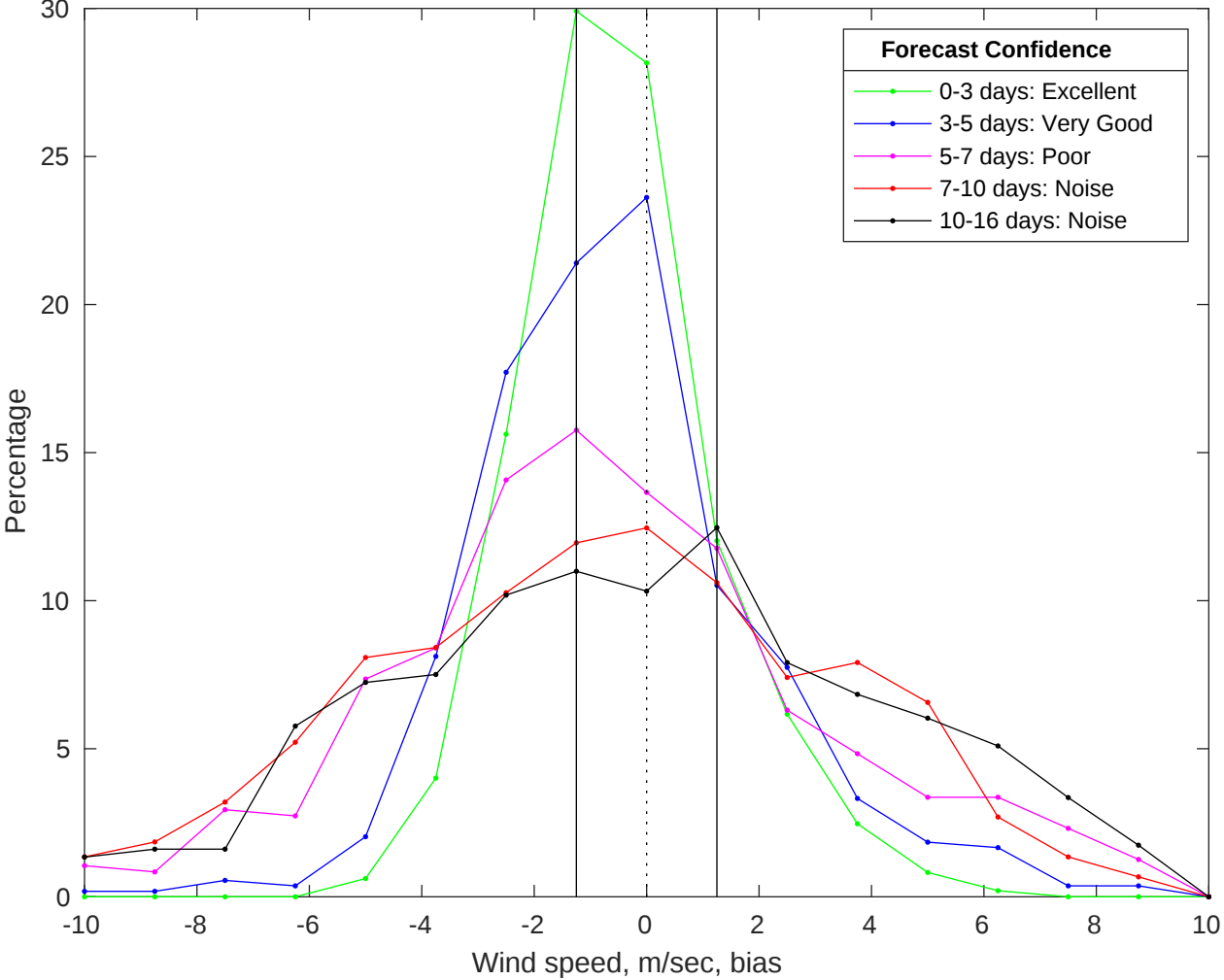
NDBC 41004 vs GFS Winds Bias Histogram: 02-Jan-2026
