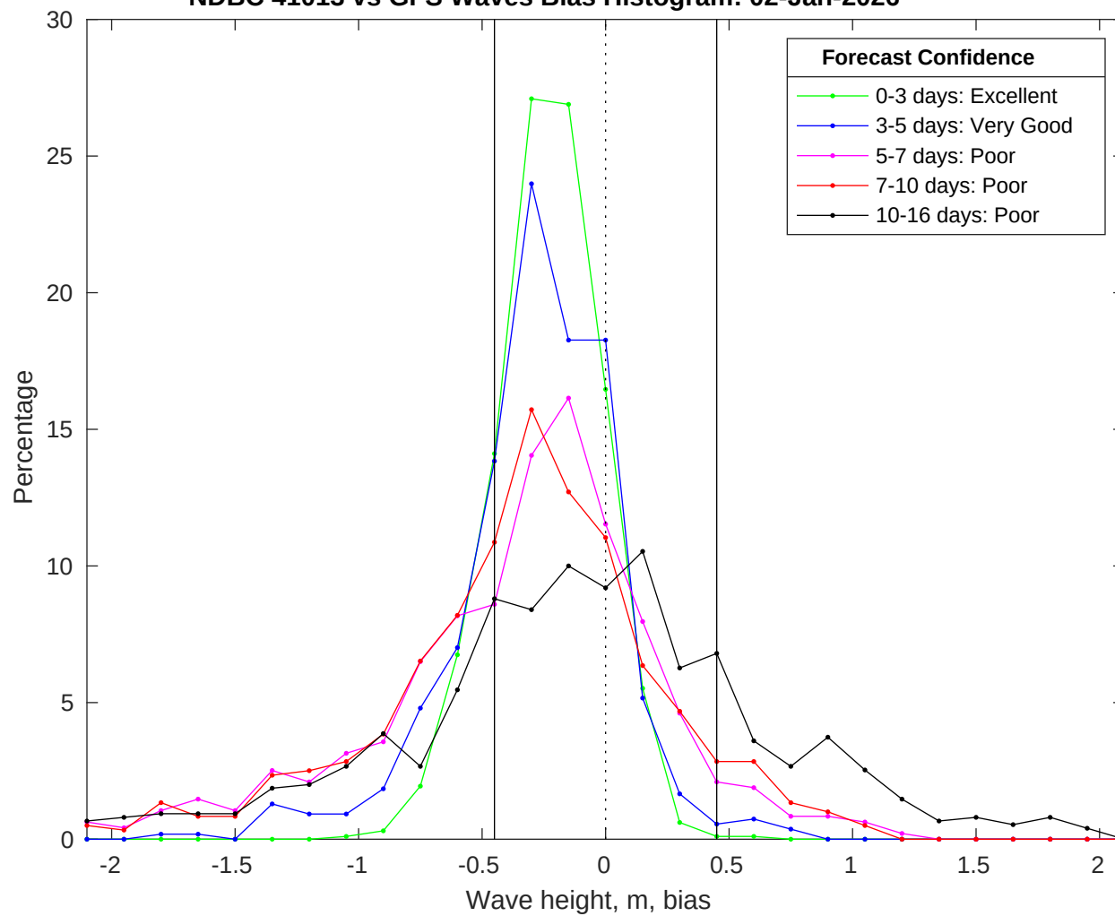
NDBC 41013 vs GFS Waves Bias Histogram: 02-Jan-2026
