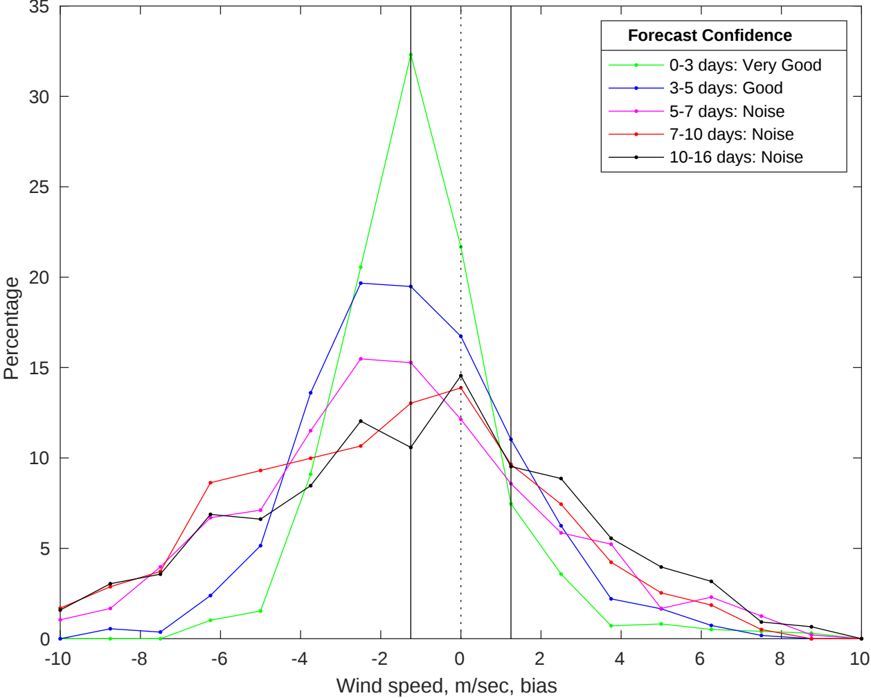
NDBC 41013 vs GFS Winds Bias Histogram: 02-Jan-2026
