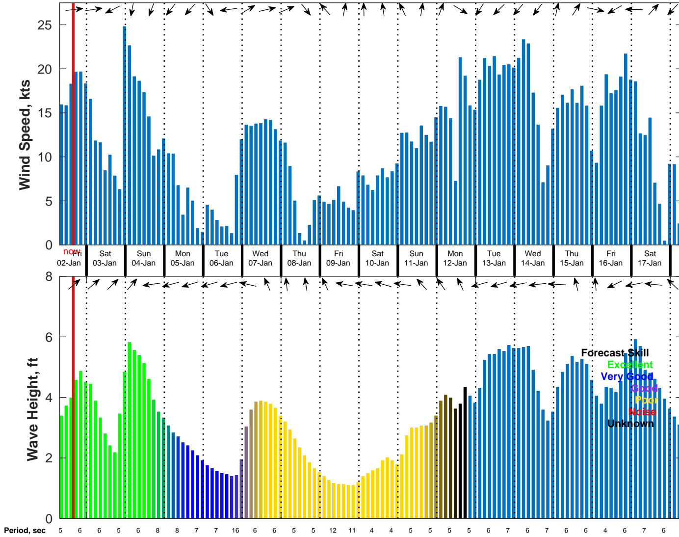
Wind & Wave Forecast for NDBC 41013 from 02-Jan-2026 07:00:00 to 18-Jan-2026 07:00:00
