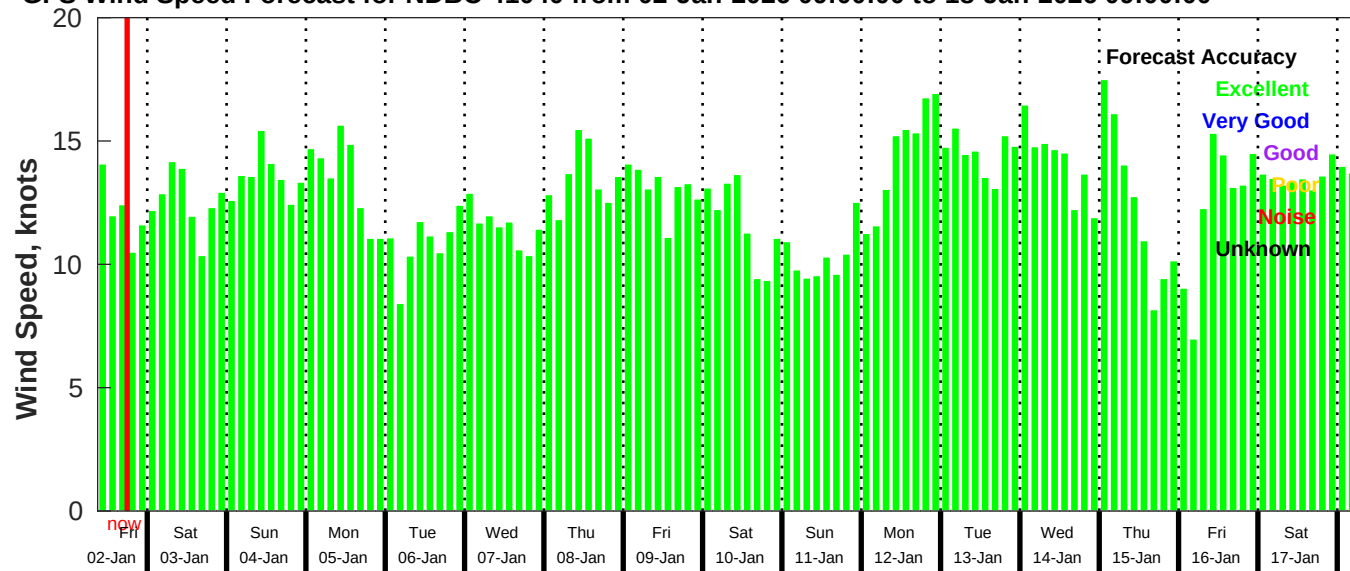
GFS Wind Speed Forecast for NDBC 41040 from 02-Jan-2026 09:00:00 to 18-Jan-2026 09:00:00
