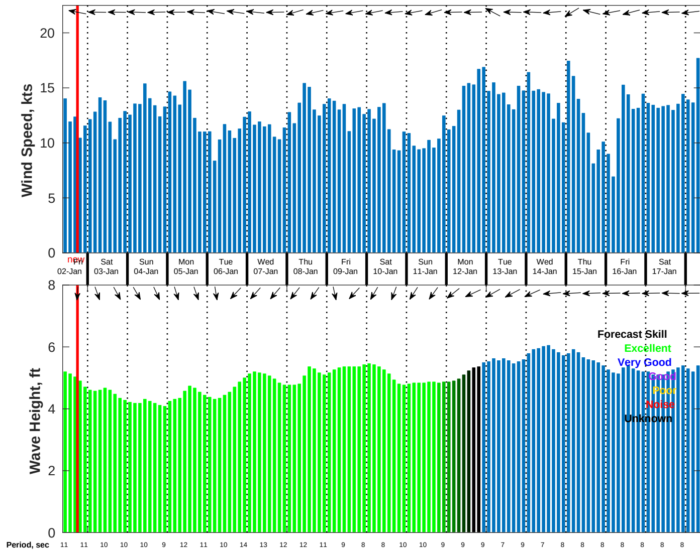
Wind & Wave Forecast for NDBC 41040 from 02-Jan-2026 09:00:00 to 18-Jan-2026 09:00:00
