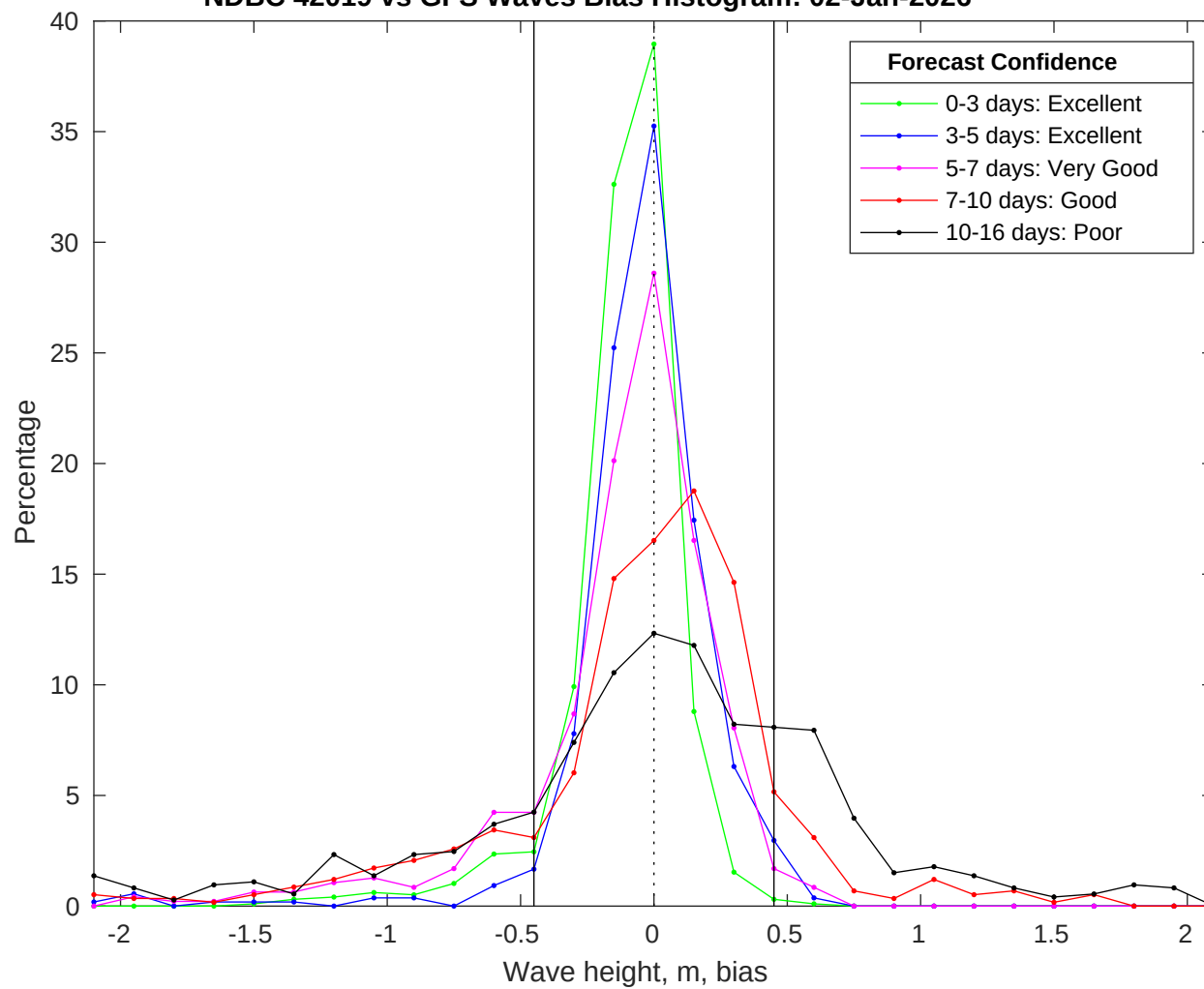
NDBC 42019 vs GFS Waves Bias Histogram: 02-Jan-2026
