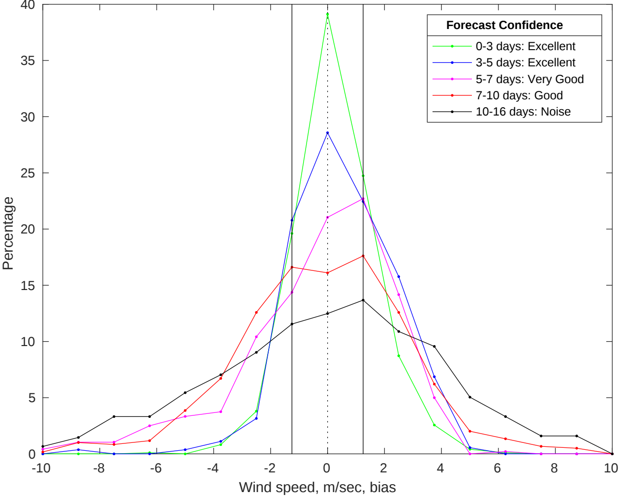
NDBC 42019 vs GFS Winds Bias Histogram: 02-Jan-2026
