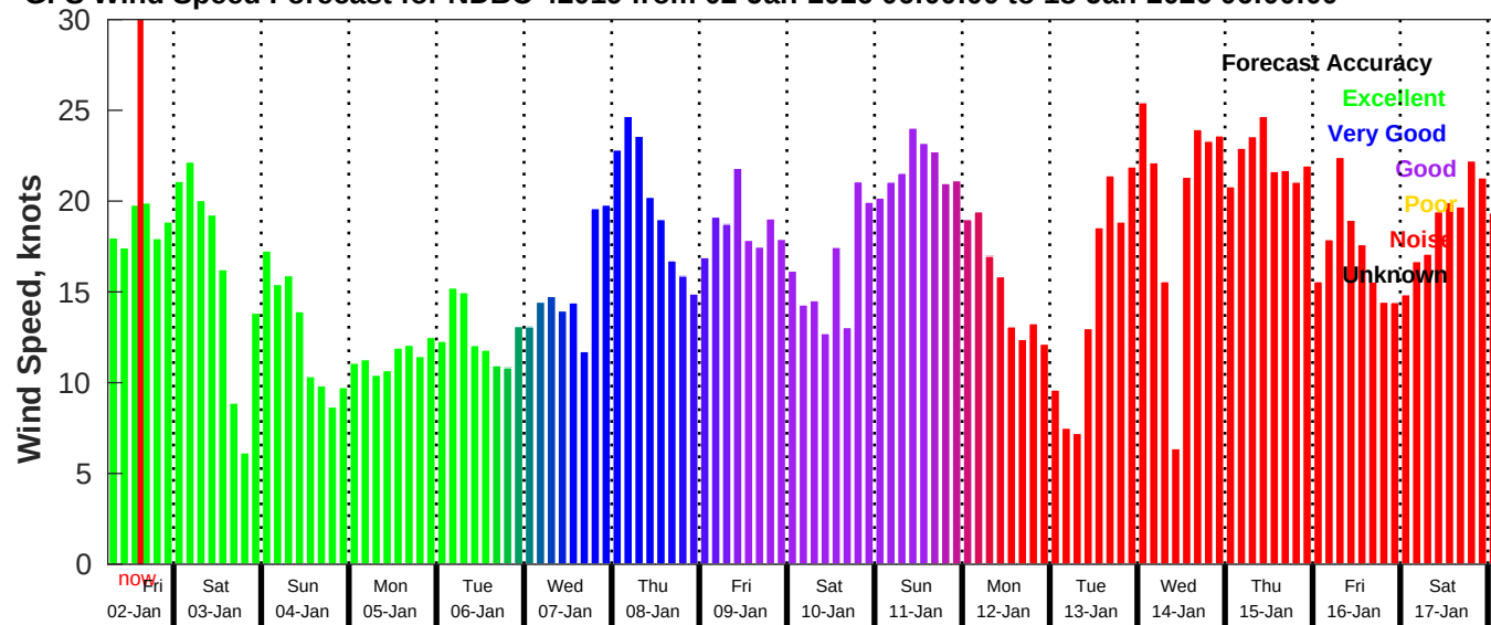
GFS Wind Speed Forecast for NDBC 42019 from 02-Jan-2026 06:00:00 to 18-Jan-2026 06:00:00
