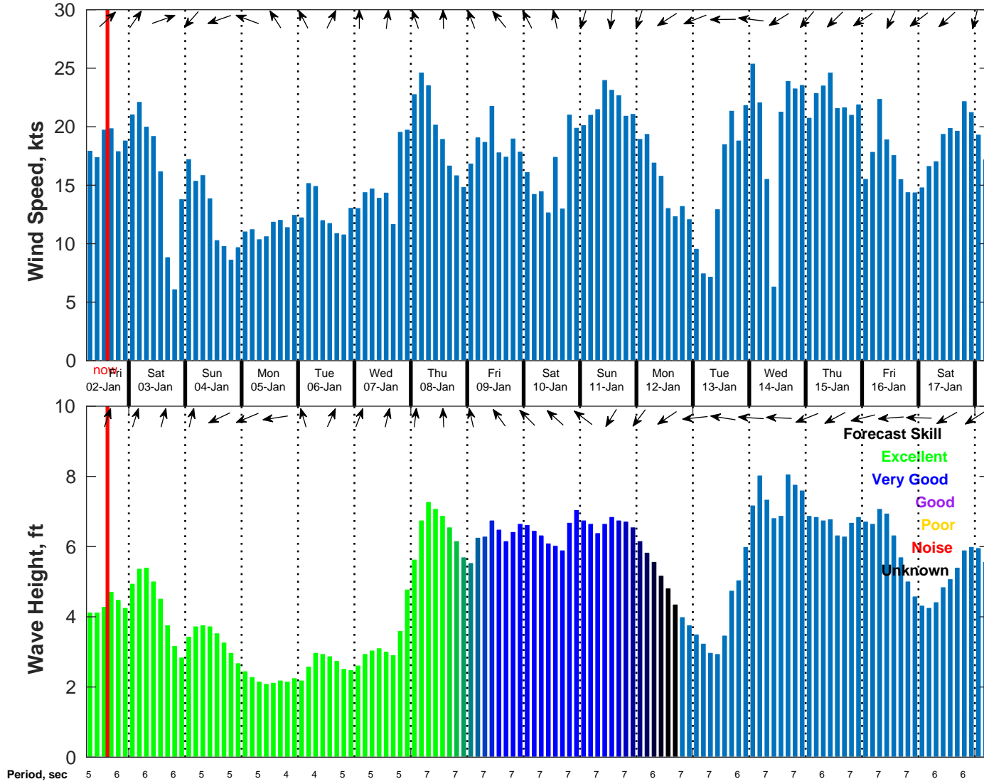
Wind & Wave Forecast for NDBC 42019 from 02-Jan-2026 06:00:00 to 18-Jan-2026 06:00:00
